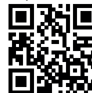
QR Gymkhana
